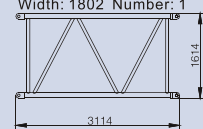
3m main boom intermediate section: 0.386t Width: 1802 Number: 1
