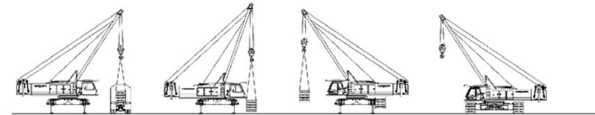
Unloading and assembly of crawler carriers
