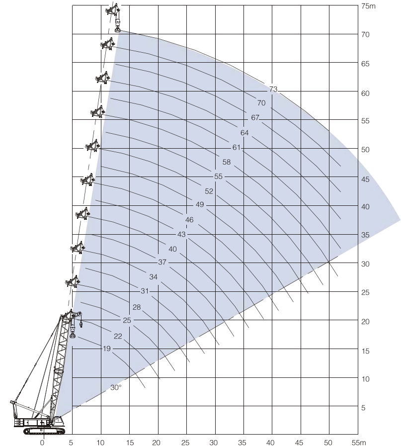
Lifting height on S boom
