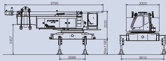
Crawler carrier: 13.68t Number: 2
